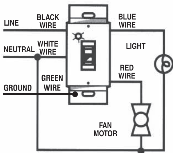
FAN/LIGHT WIRING
