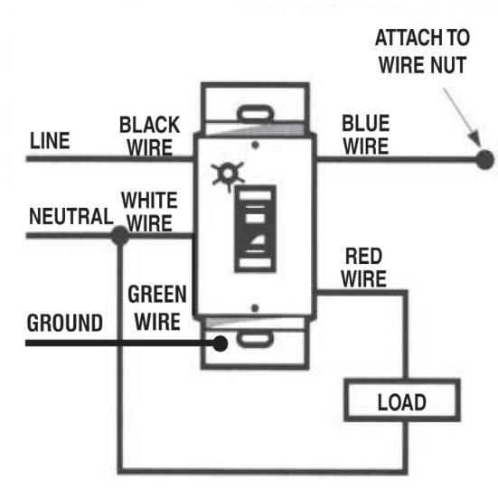
SINGLE LOAD WIRING
